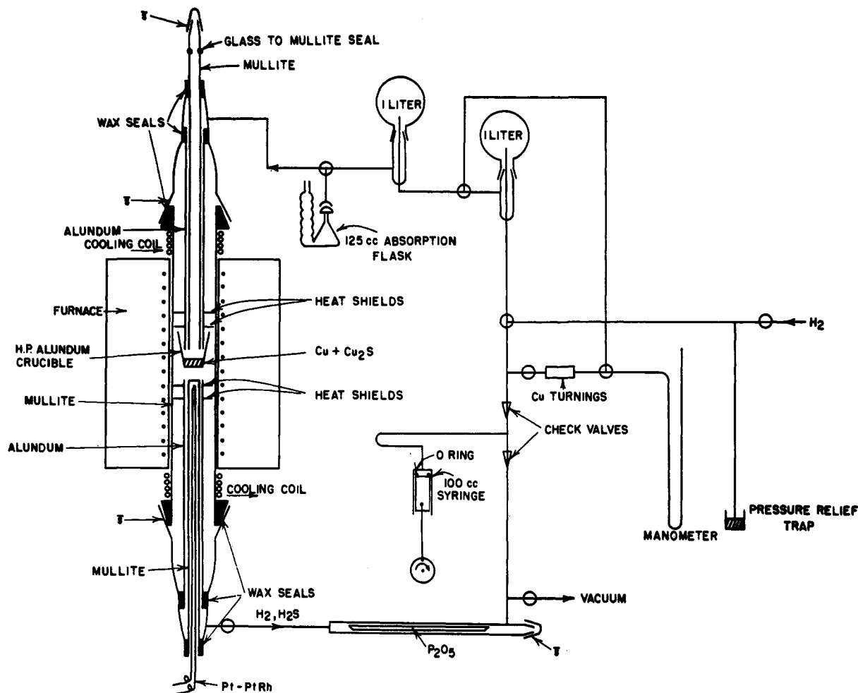
Fig. 1.—Schematic diagram of apparatus.
